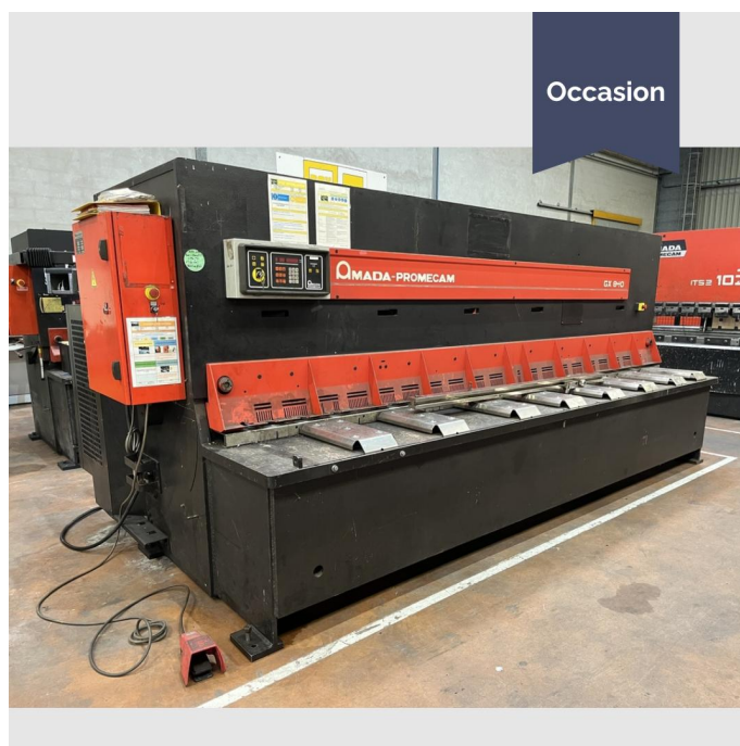
Cisaille Guillotine GX 840 GE - AMADA.webp
